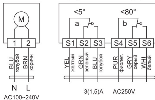
RLF03-220S(H), RLF05-220S(H)
